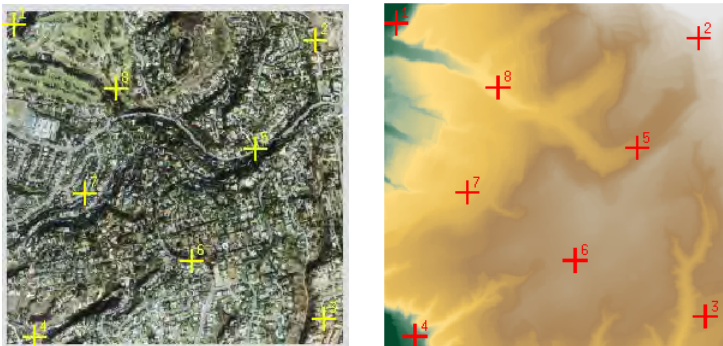
A well-distributed set of ground control points for the IKONOS multispectral image of La Jolla Mesa (left) covers the image extents and also includes a range of elevations, as shown in the view of the DEM (right).
