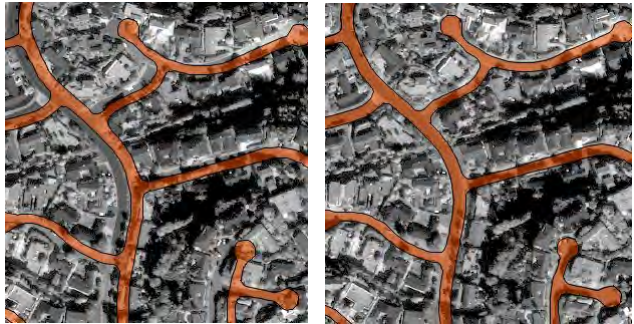
Planimetric street vector (orange, traced from aerial orthophoto) overlaid on panchromatic IKONOS satellite image (1-meter cell size) of part of La Jolla, California. Left, georeferenced but unrectified image. Right, image after RPC orthorectification, resulting in excellent match with street vector. Area has about 60 meters of relief.
