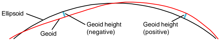
Geoid height in vertical section (exaggerated)
